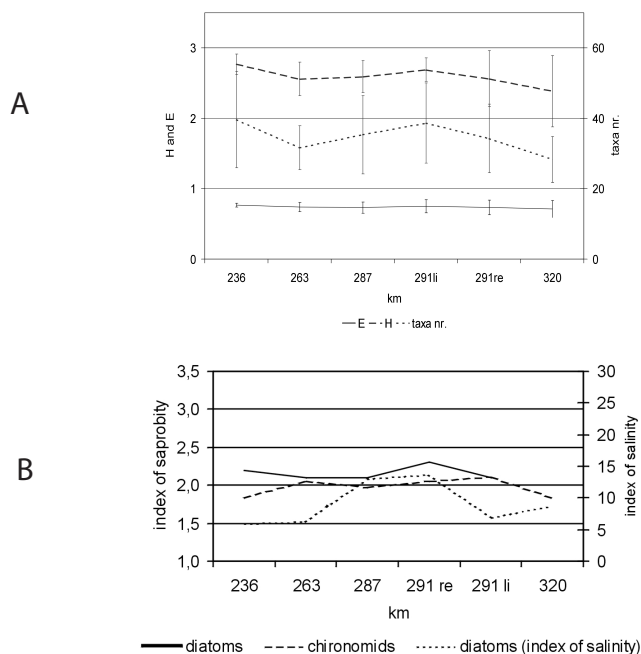
Fig. 1. A: Evenness (E), Shannon Wiener index (H), and taxa richness of the chironomid communities (average of 3 dates and standard errors). B: Indices of saprobity calculated from the chironomid and diatom communities, and indices of salinity (diatoms) at the stations studied (river km).
