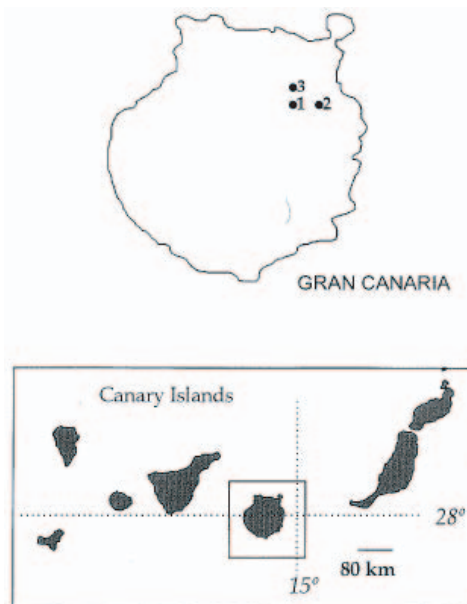
Fig. 1 - Map of Gran Canaria (Canary Islands) showing location of sampling sites. 1: Tafira Alta; 2: Jinamar; 3: San Lorenzo.
