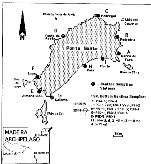
Figure 1 - Porto Santo Island: Benthos sampling stations
