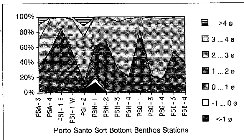
Figure 2 - Porto Santo: Grain-size Distribution per Station. Wentworth PHI scale - Ø: Mud: >4 Ø; very fine sand: 3... 4 Ø; fine sand: 2 to 3 Ø; medium sand: 1 to 2 Ø; coarse sand: 0 to 1 Ø; very coarse sand: -1 to 0 Ø; Gravel: <-1 Ø.
