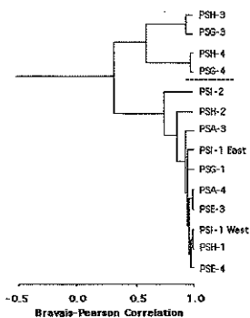
Figure 9 - Stations grouping (cluster analysis - Q mode), based on the values of sediment parameters and taxa , per station.
