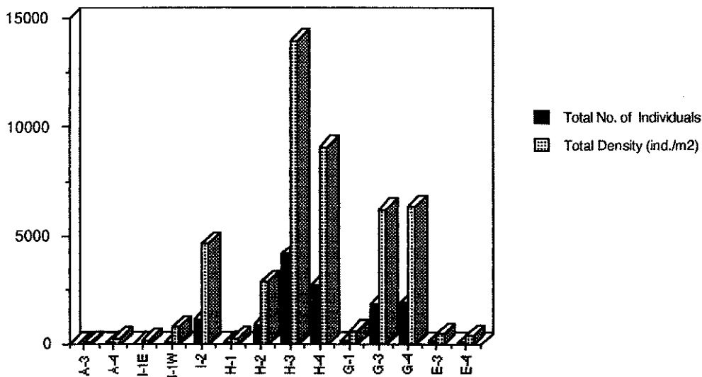
Figure 6 - Variation of soft bottom macrofauna: number of individuals and densities per station.
